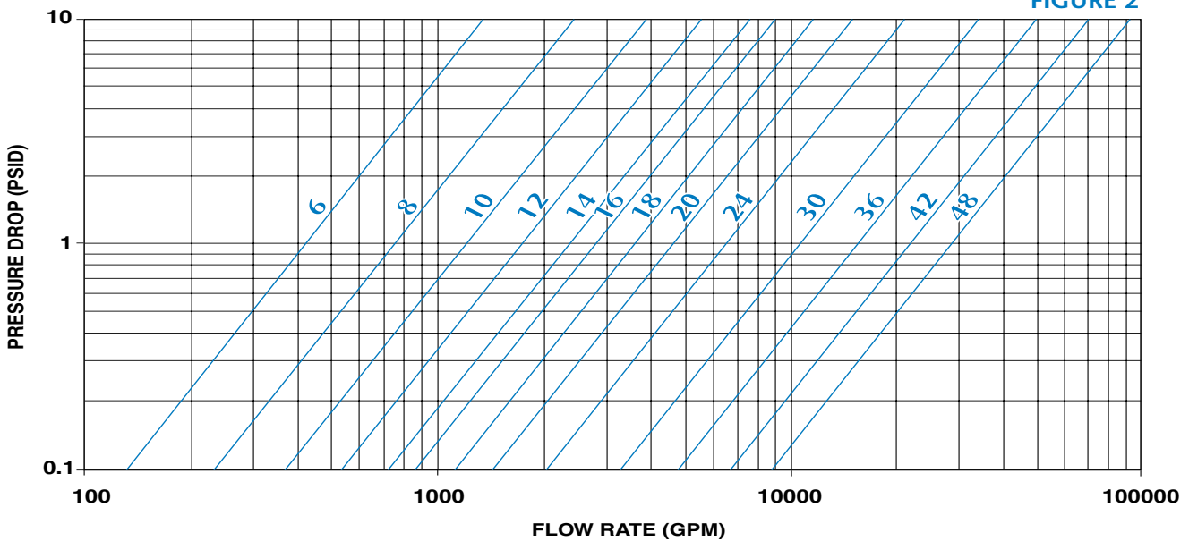
TEMPORARY STRAINER PRESSURE DROP - LIQUIDS (SIZES 6" - 48")
