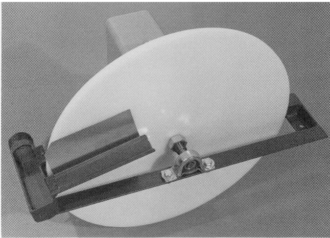
18" one wheel side discharge skimmer Model 28150
