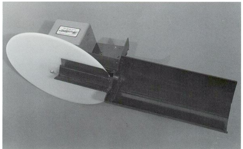
12" one wheel front discharge skimmer Model 12151
