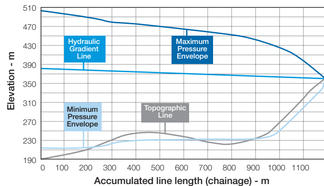
Line Hydraulic Behavior without Protection
