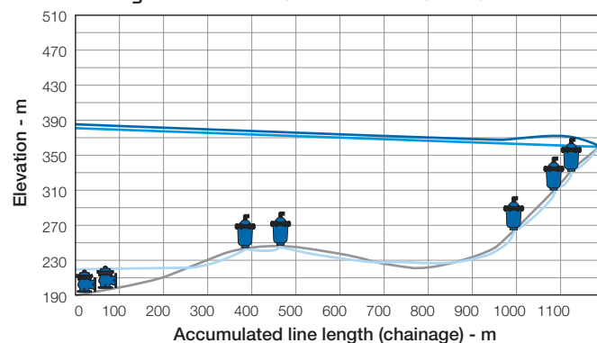
Line Hydraulic Behavior with Full Protection
