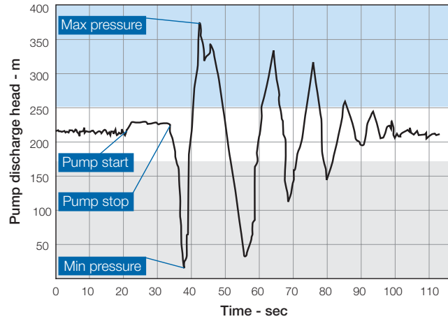
Surge at Pump Station Without Protection
