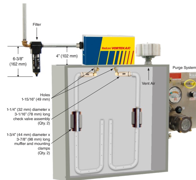
HAZARDOUS LOCATION VORTEX A/C (MODEL 7570 SHOWN TOP MOUNTED ON CUSTOMER'S ENCLOSURE) (PURGE SYSTEM SHOWN FOR REFERENCE ONLY)
